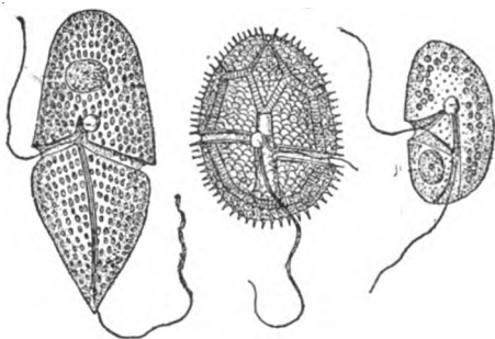
FIG. 281.—Typical forms of the Peridinea ; \times about 500.
